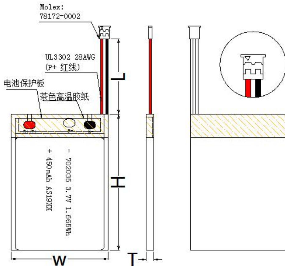
Fig.2 Dimensional Drawing of AS 702035 电池包规格尺寸
